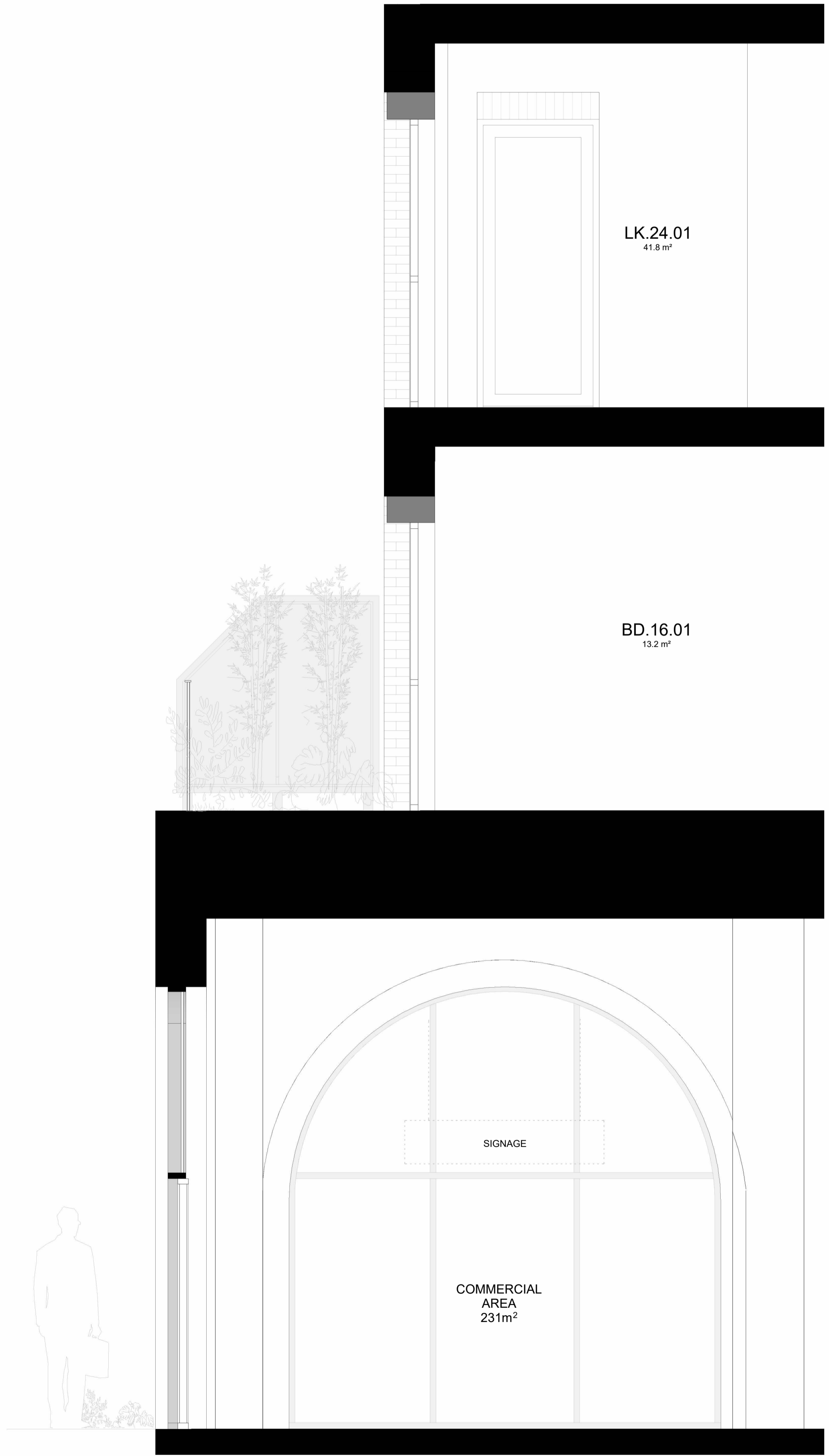
2 Commercial Arch Section SCALE 1:25
