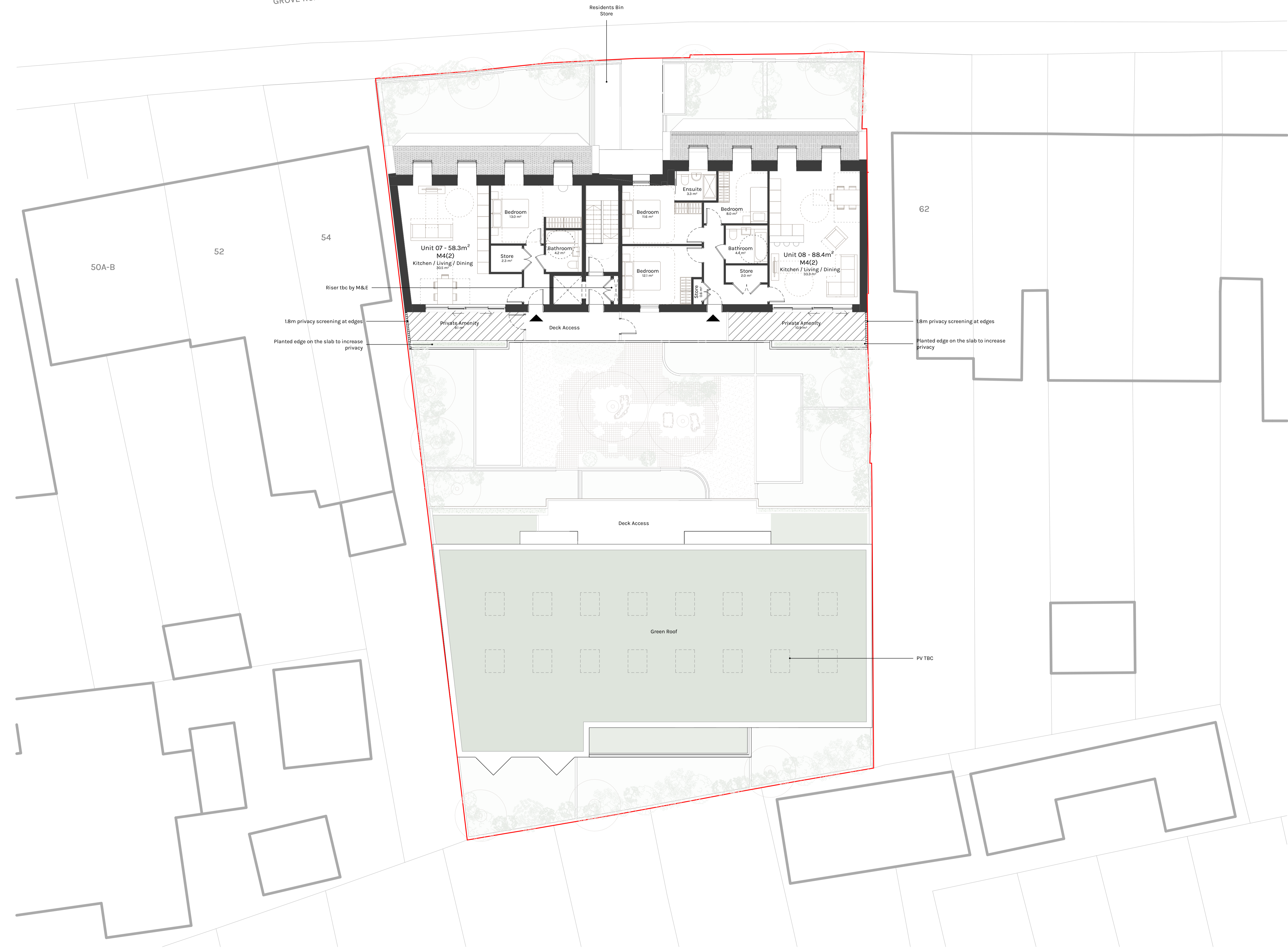
1 Second Floor Plan 1:100
