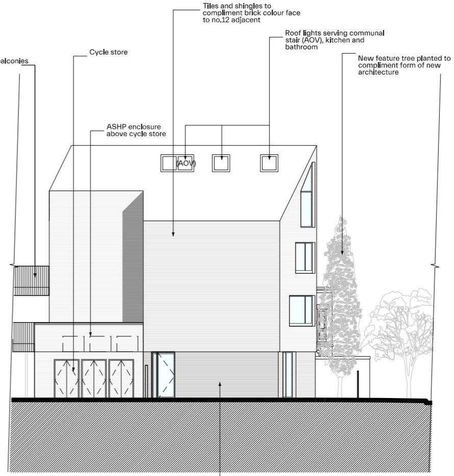
Block B Proposed Elevation C (Side)
