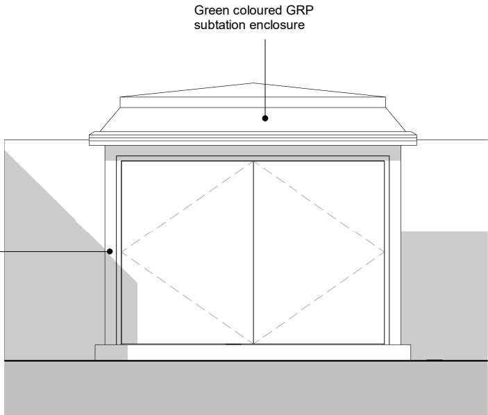
Front Elevation 3 1 : 50
