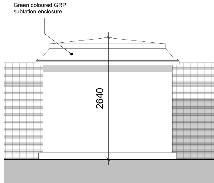
West Elevation 6 1 : 50
