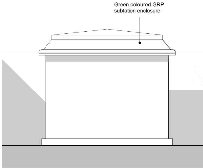
East Elevation 4 1 : 50
