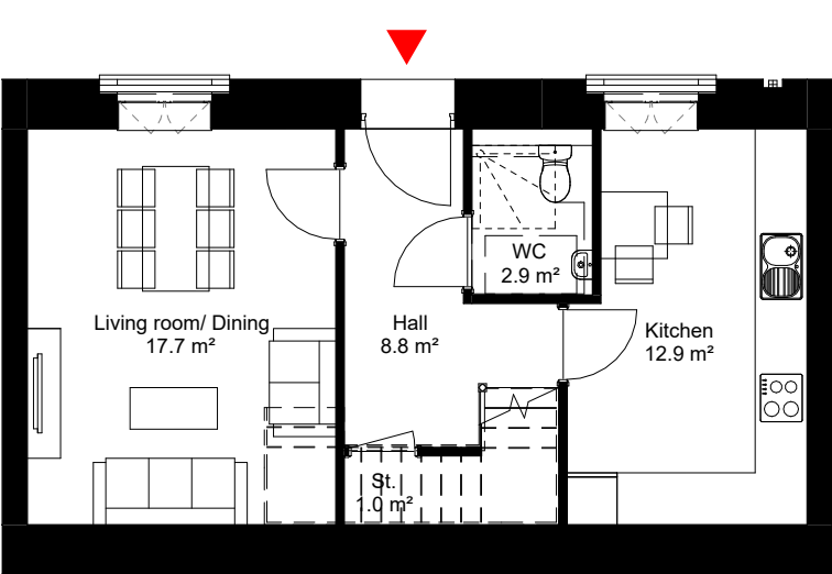
Proposed Dwelling Type - H13604 Level 0 1 : 100
