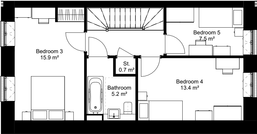
Proposed Dwelling Type - H15801 Level 2 1 : 100
