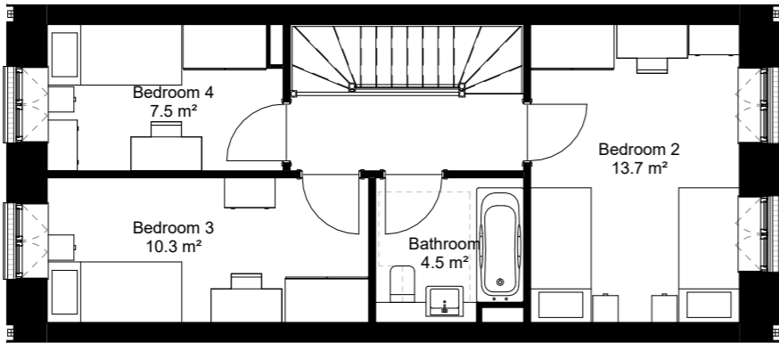
Proposed Dwelling Type - H14601 Level 1 1 : 100
