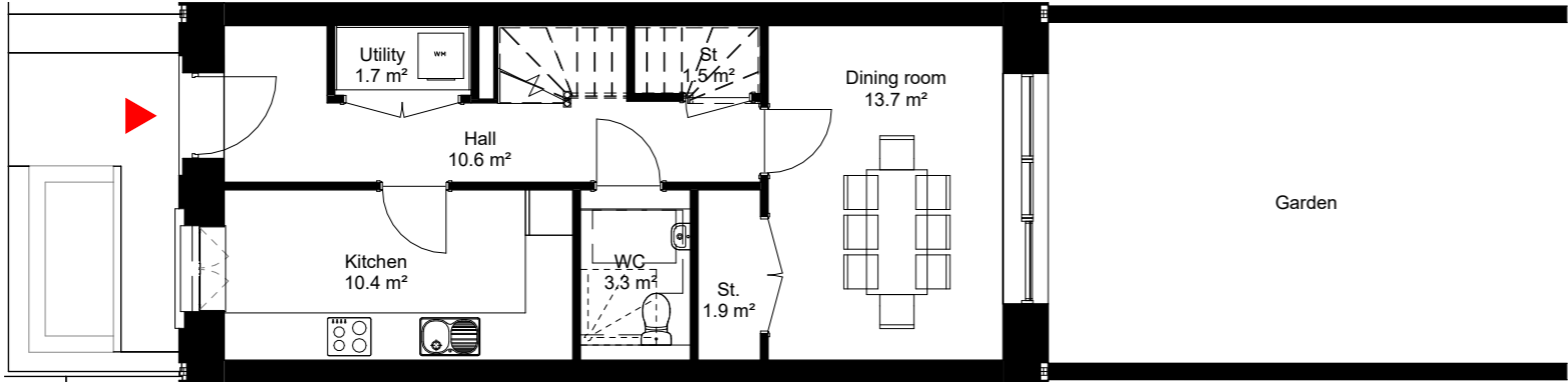
Proposed Dwelling Type - H14601 Level 0 1 : 100
