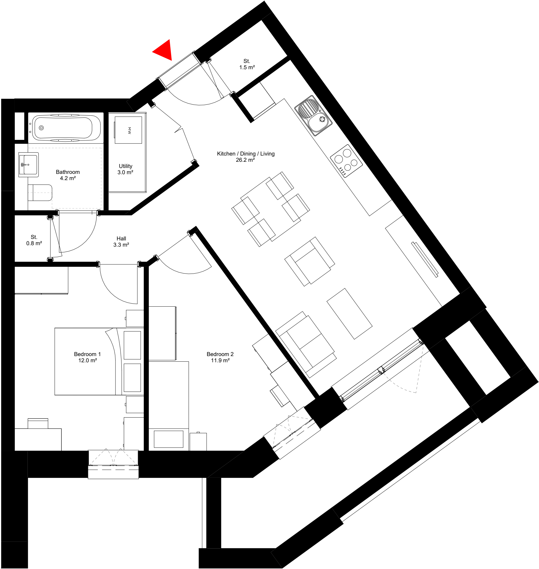
Proposed Dwelling Type - P2307 1 : 50
