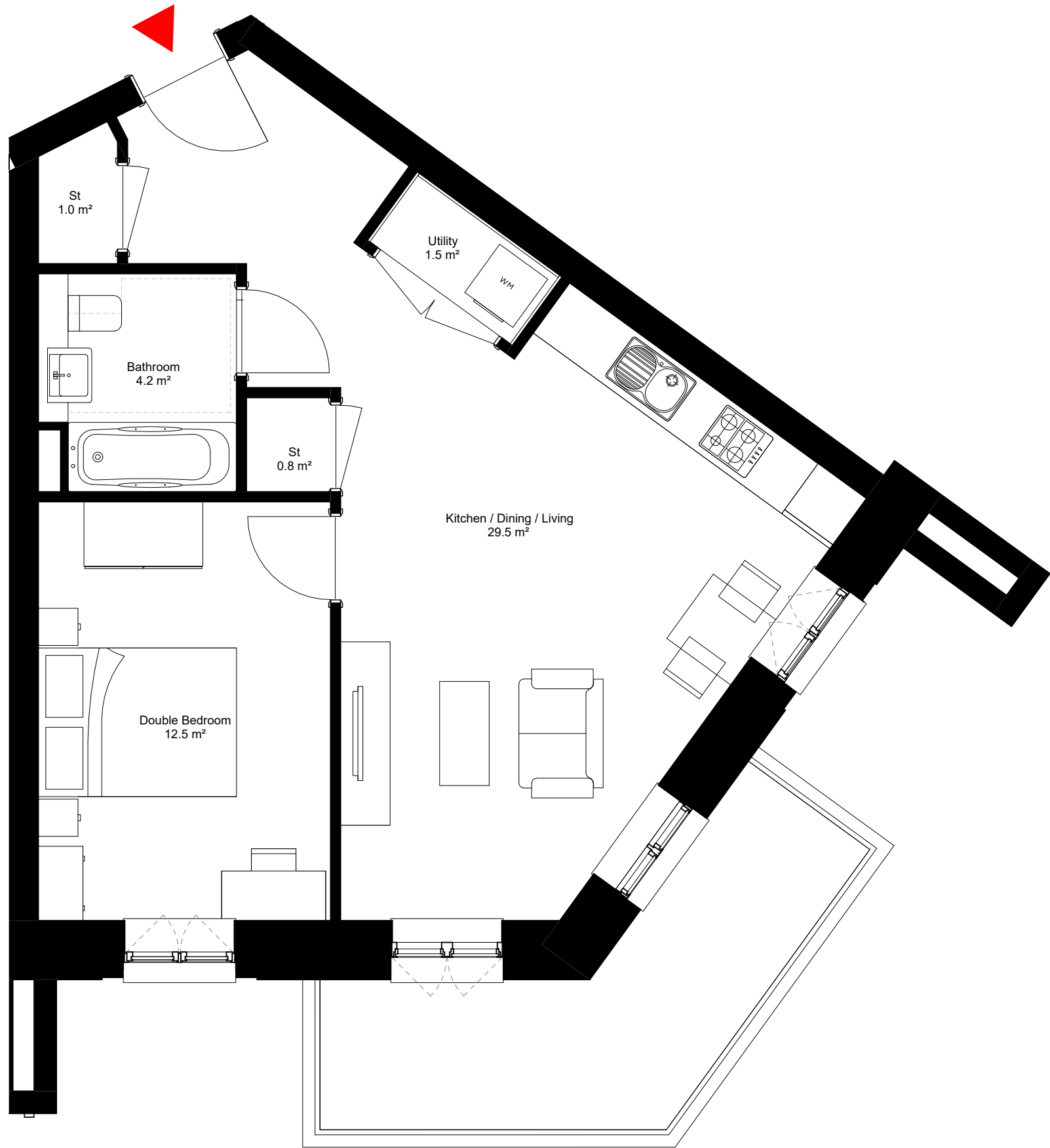
Proposed Dwelling Type - P1203 1 : 50
