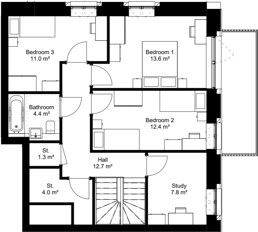
Proposed Dwelling Type - A3509 Level 1 1 : 100
