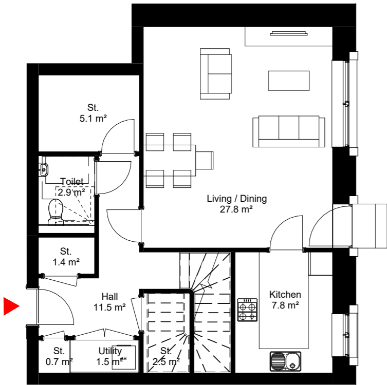
Proposed Dwelling Type - A3509 Level 0 1 : 100
