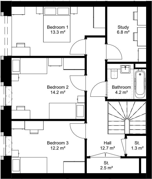
Proposed Dwelling Type - A3507 Level 1 1 : 100
