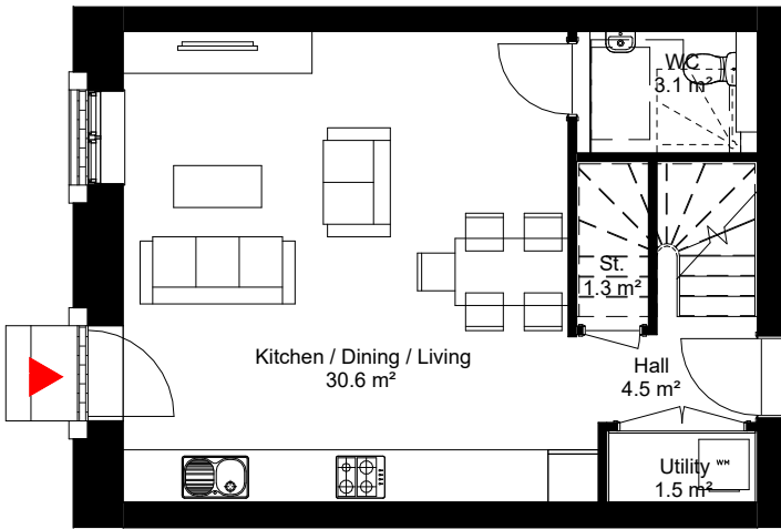
Proposed Dwelling Type - A3507 Level 0 1 : 100
