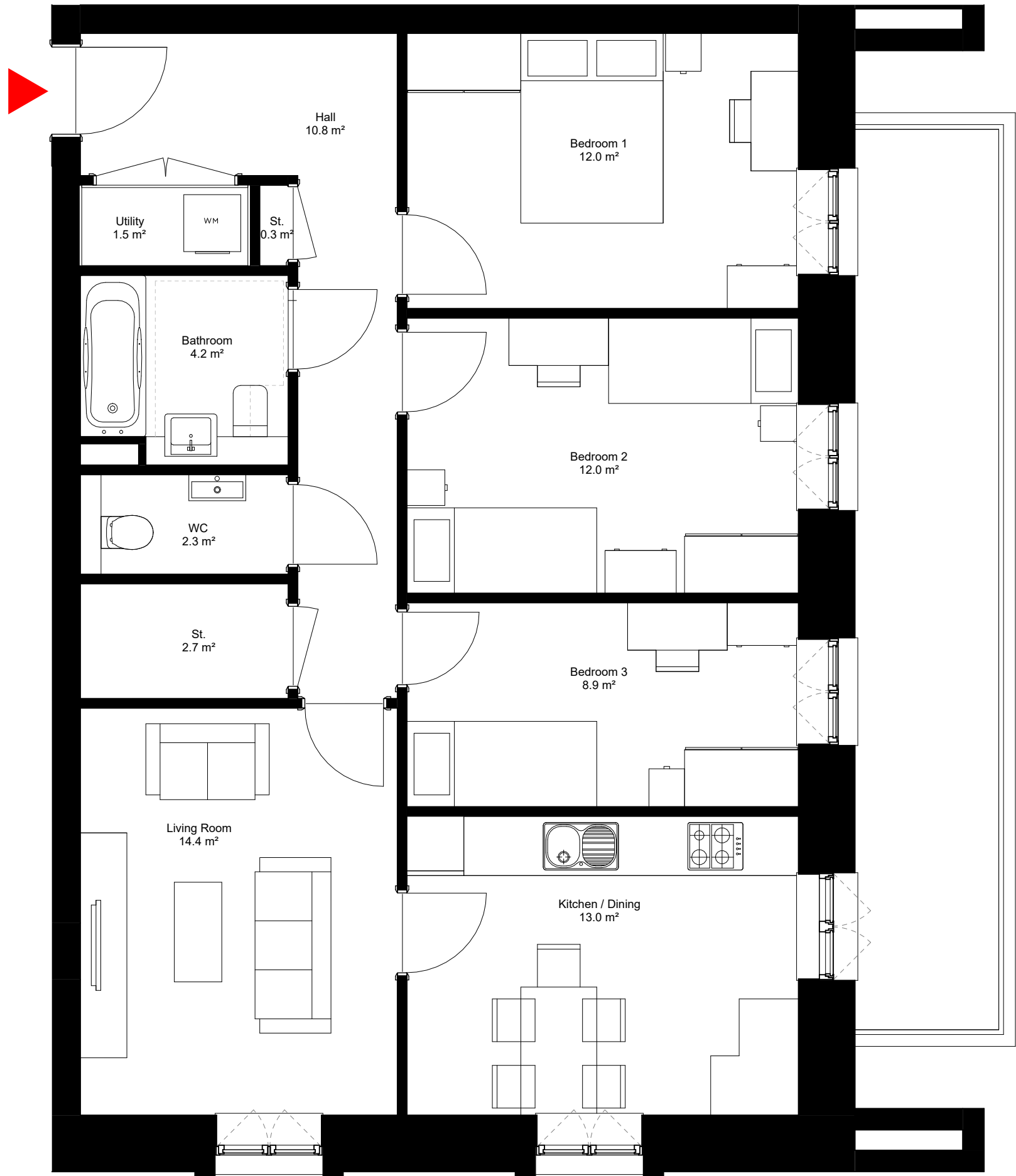
Proposed Dwelling Type - A3506 1 : 50
