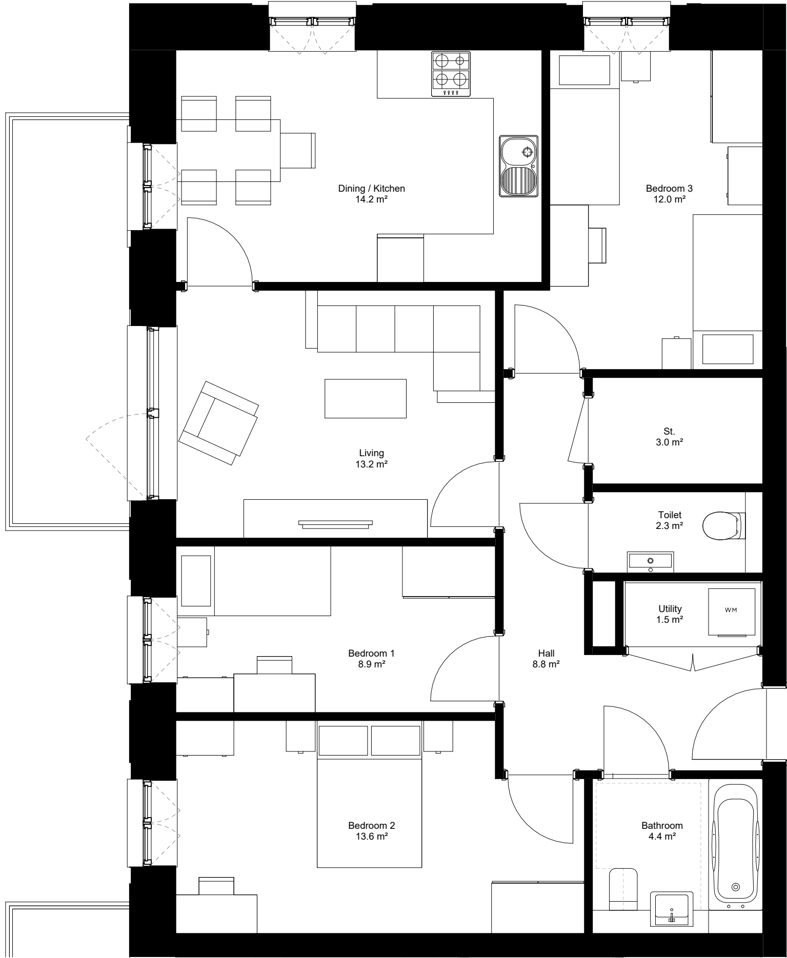
Proposed Dwelling Type - A3504 1 : 50
