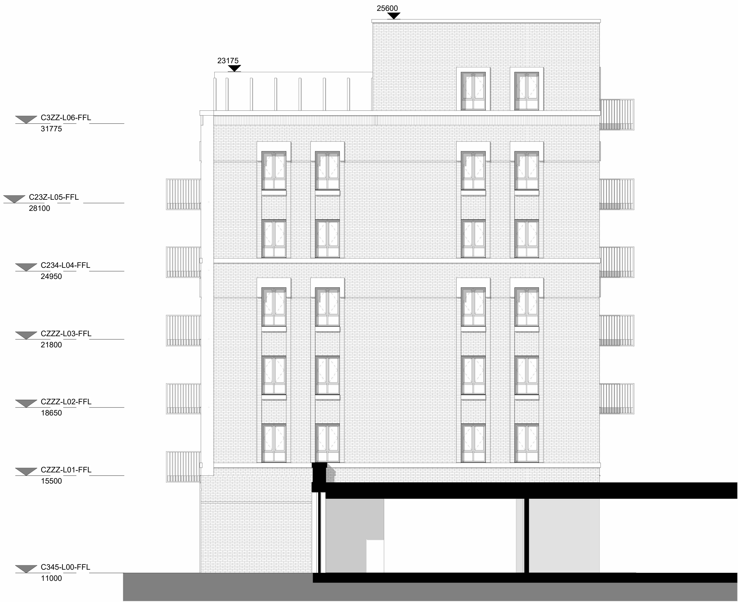
Proposed Plot C Block 3 North Elevation 1 : 100
