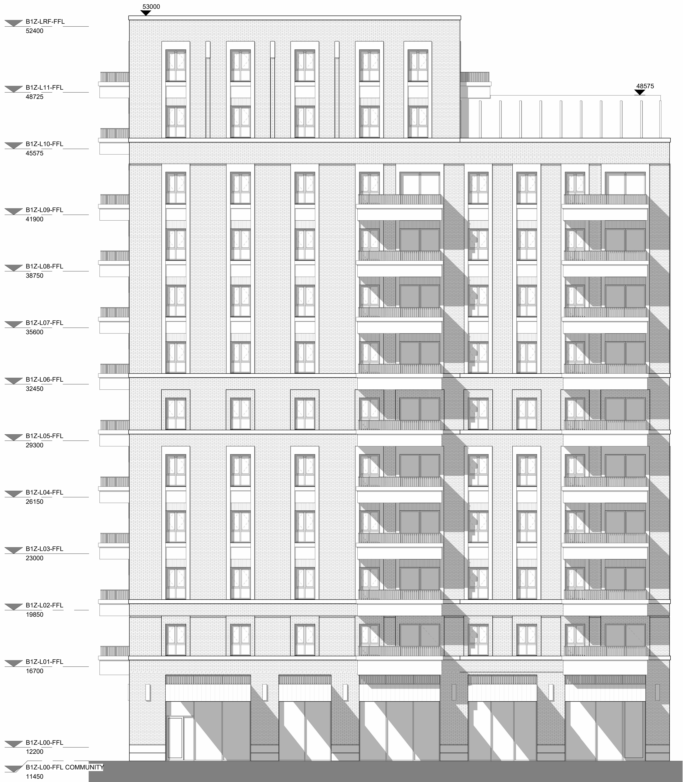
Proposed Block B01 South Elevation 1 : 100
