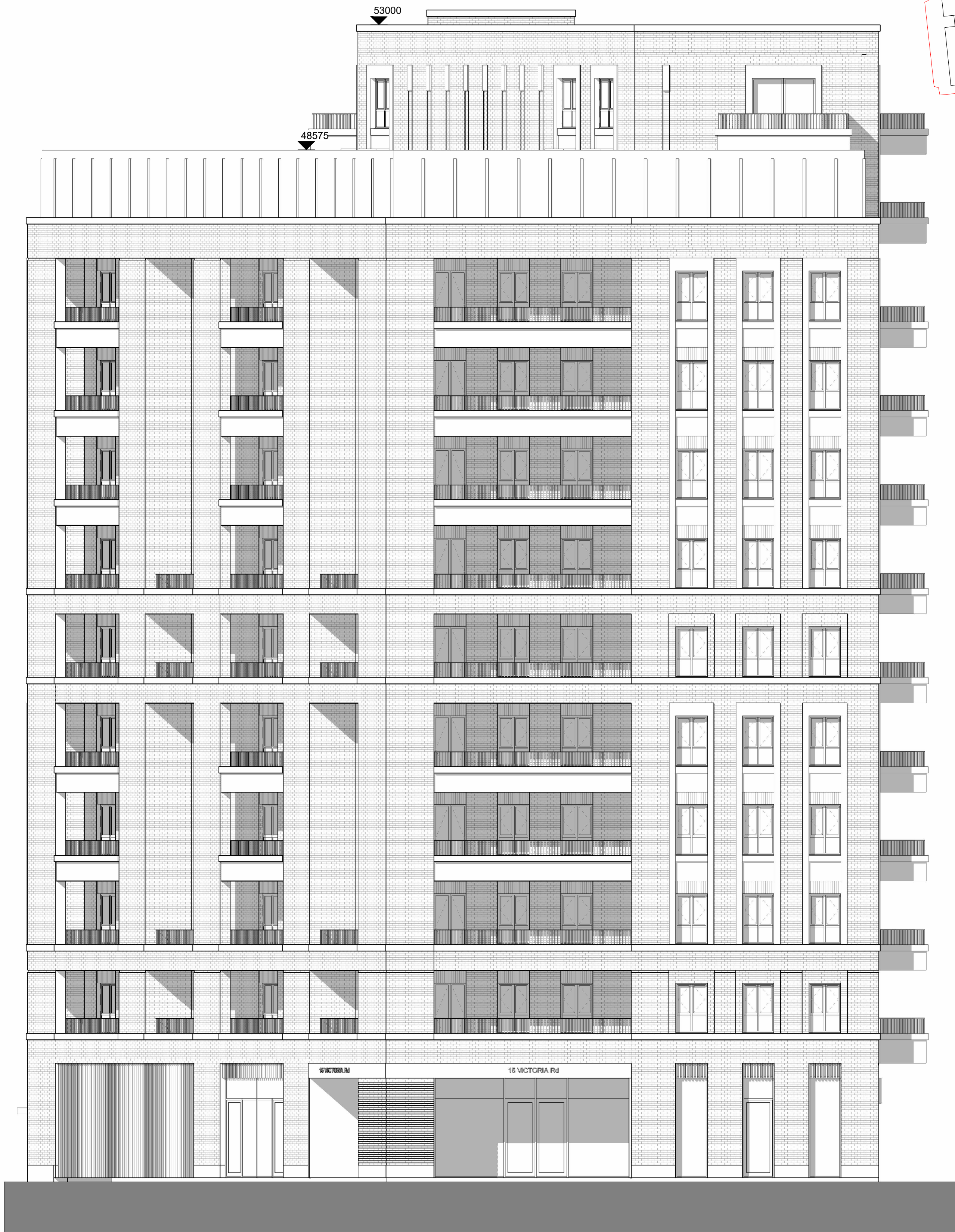
Proposed Block B01 North Elevation 1 : 100
