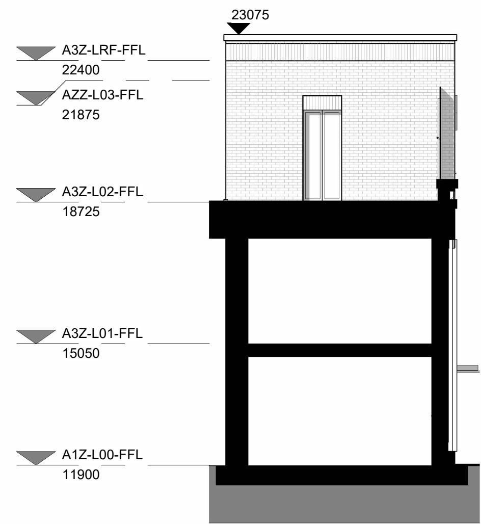
Proposed Plot A Block 3 South Elevation 1 : 100
