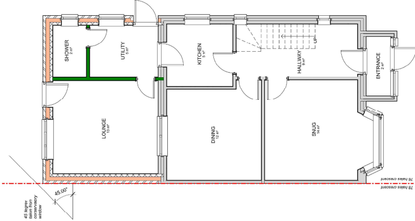
C-PROPOSED GROUND FLOOR PLAN 1:50
