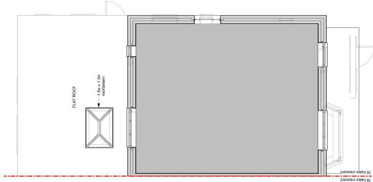
1-PROPOSED FIRST FLOOR PLAN 1:50
