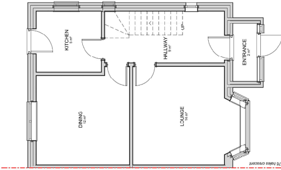
0-EXISTING GROUND FLOOR PLAN 1:50
