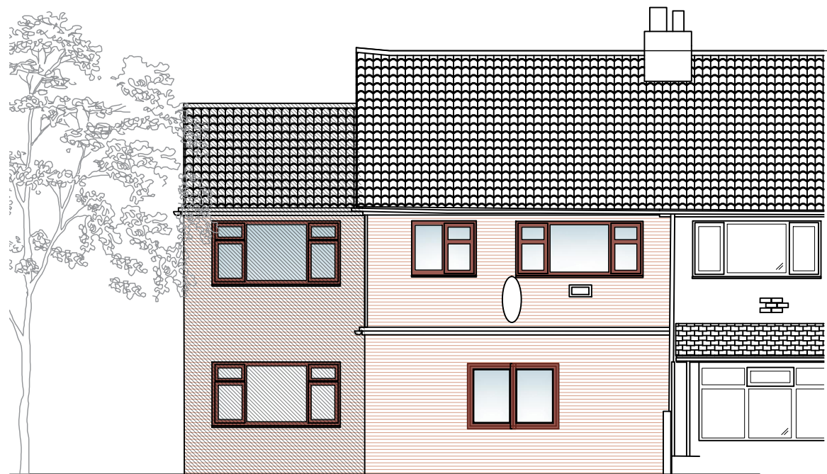
SOUTH Elevation
